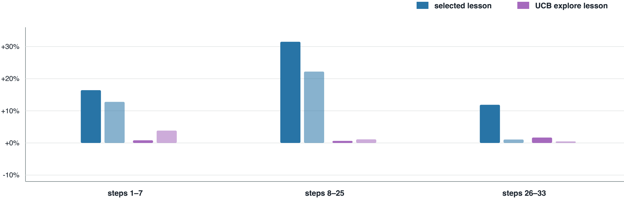
Matched best-of-13 reward uplift
